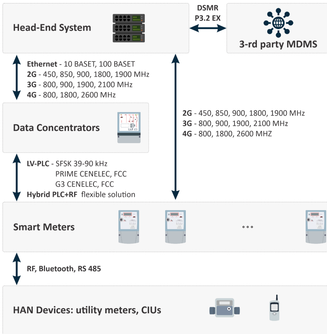
Figure 1. ADDAX Solution architecture
