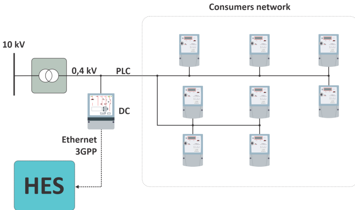
Figure 2. General scheme of data transmission via PL LV communication channel
