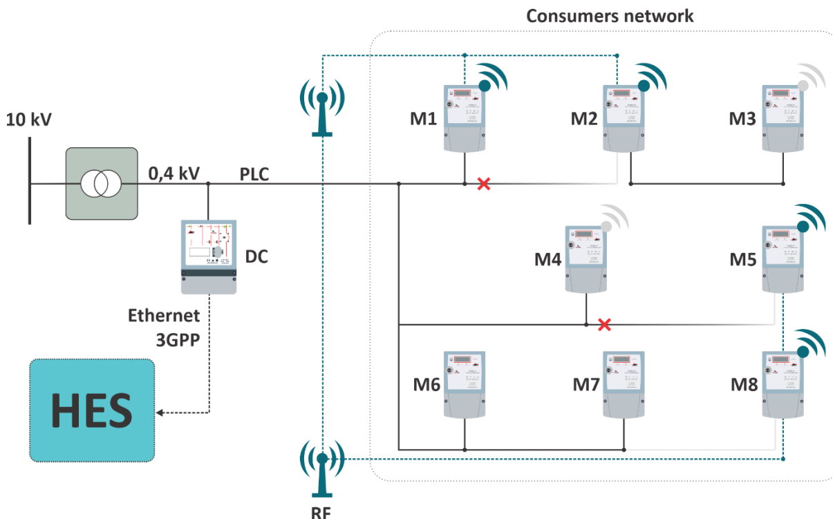
Figure 5. General scheme of data transmission via hybrid PLC+RF communication channel
